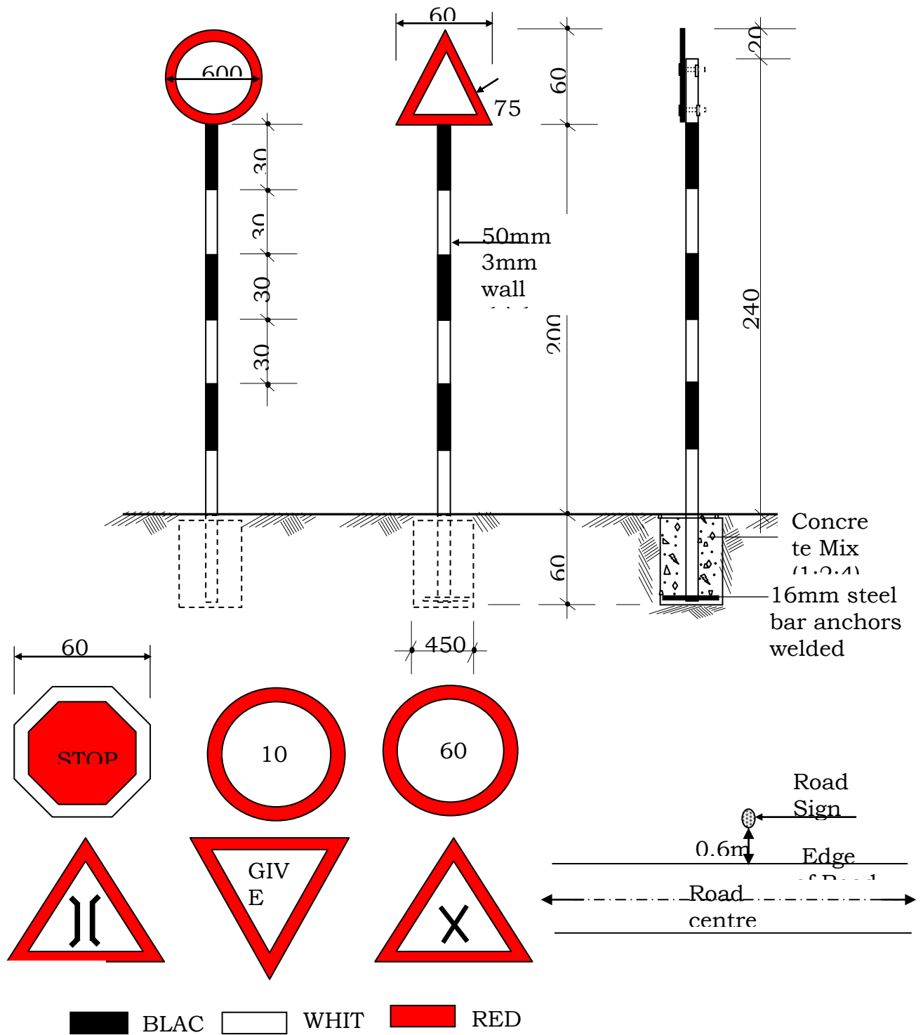
FIGURE C.16 - TRAFFIC SIGN
