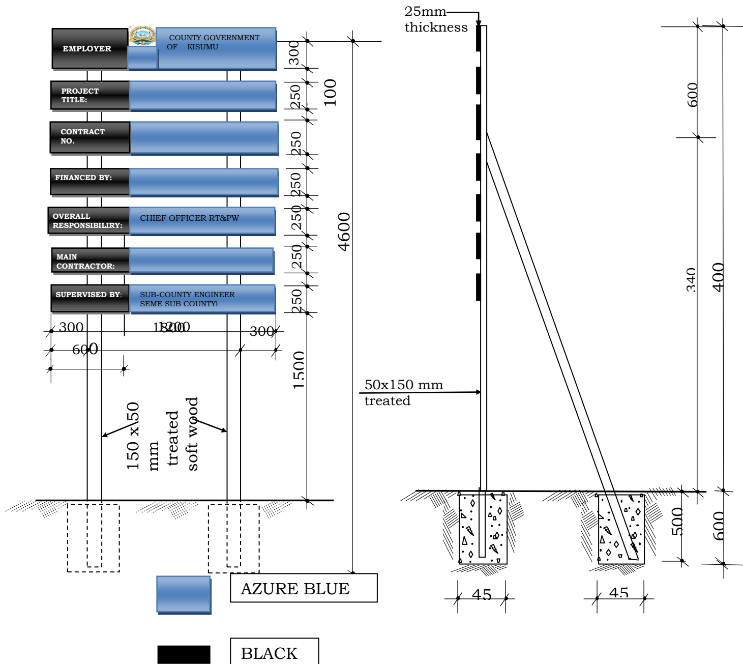
FIGURE C.20 - PUBLICITY SIGNBOARD
