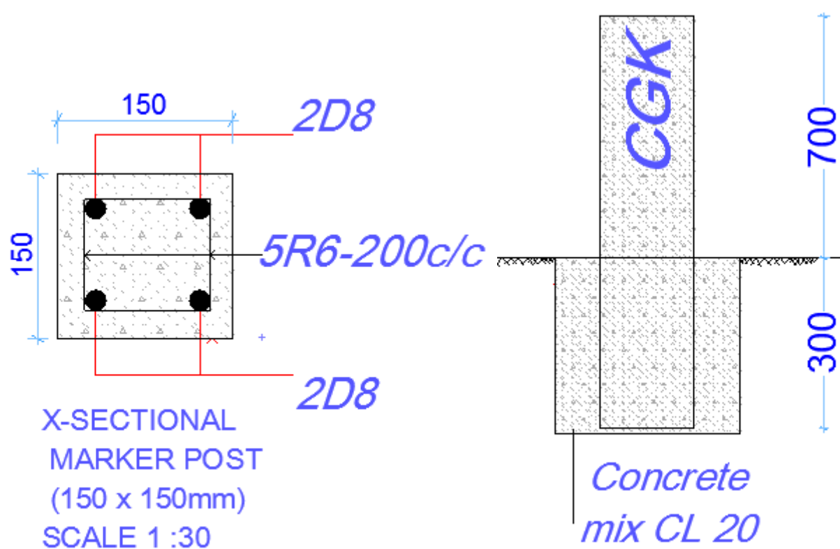
FIGURE C.18 Marker post
