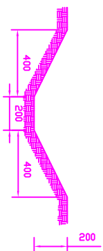
SECTION C-C
